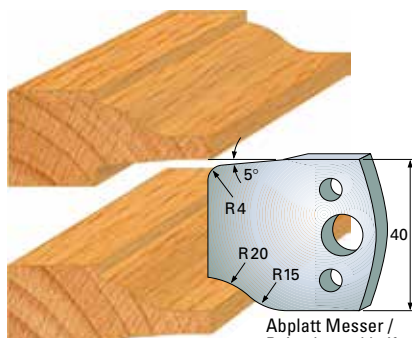
Abplatt Messer / Raised panel knife
