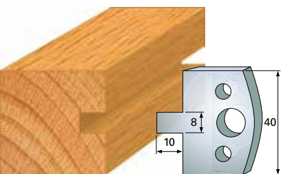
Abplatt Messer / Raised panel knife
